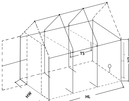
Structure Measurements
