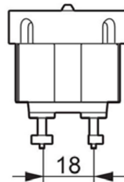
PGZ18 lamp base
