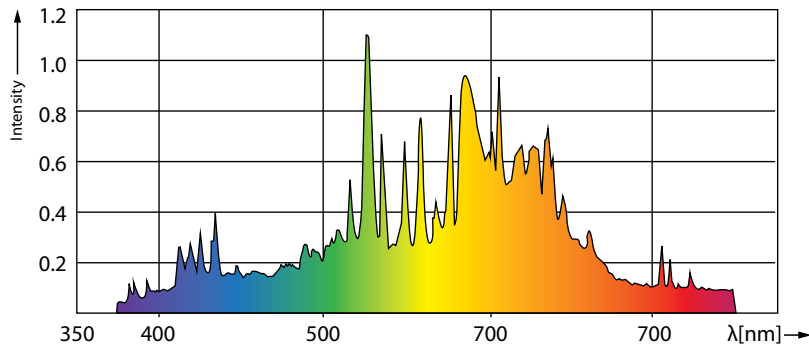
Philips 3100K - 315W Lamp (BUCMH31531K)
