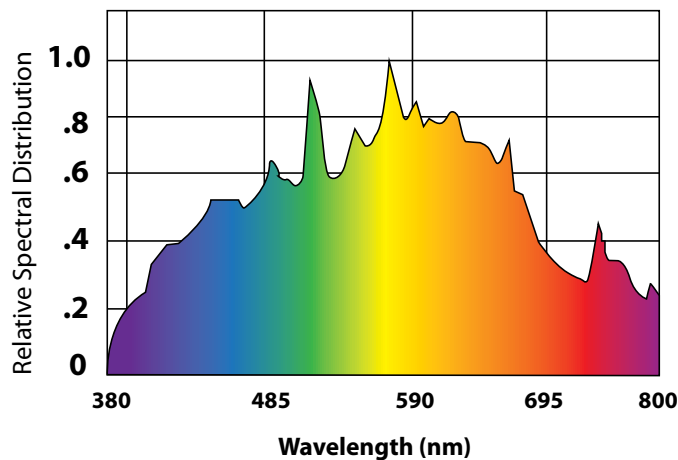
Ushio 4200K - 315W Lamp (US5002537)
