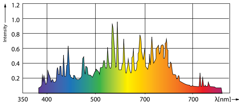
Philips 4200K - 315W Lamp (BUCMH31542K)
